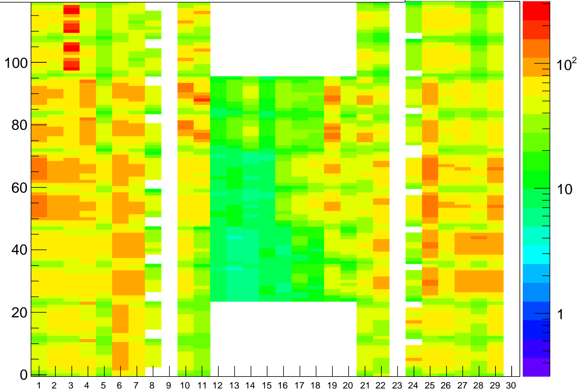
Rate (Hz) vs (BL,strip-posn), Run=19059
