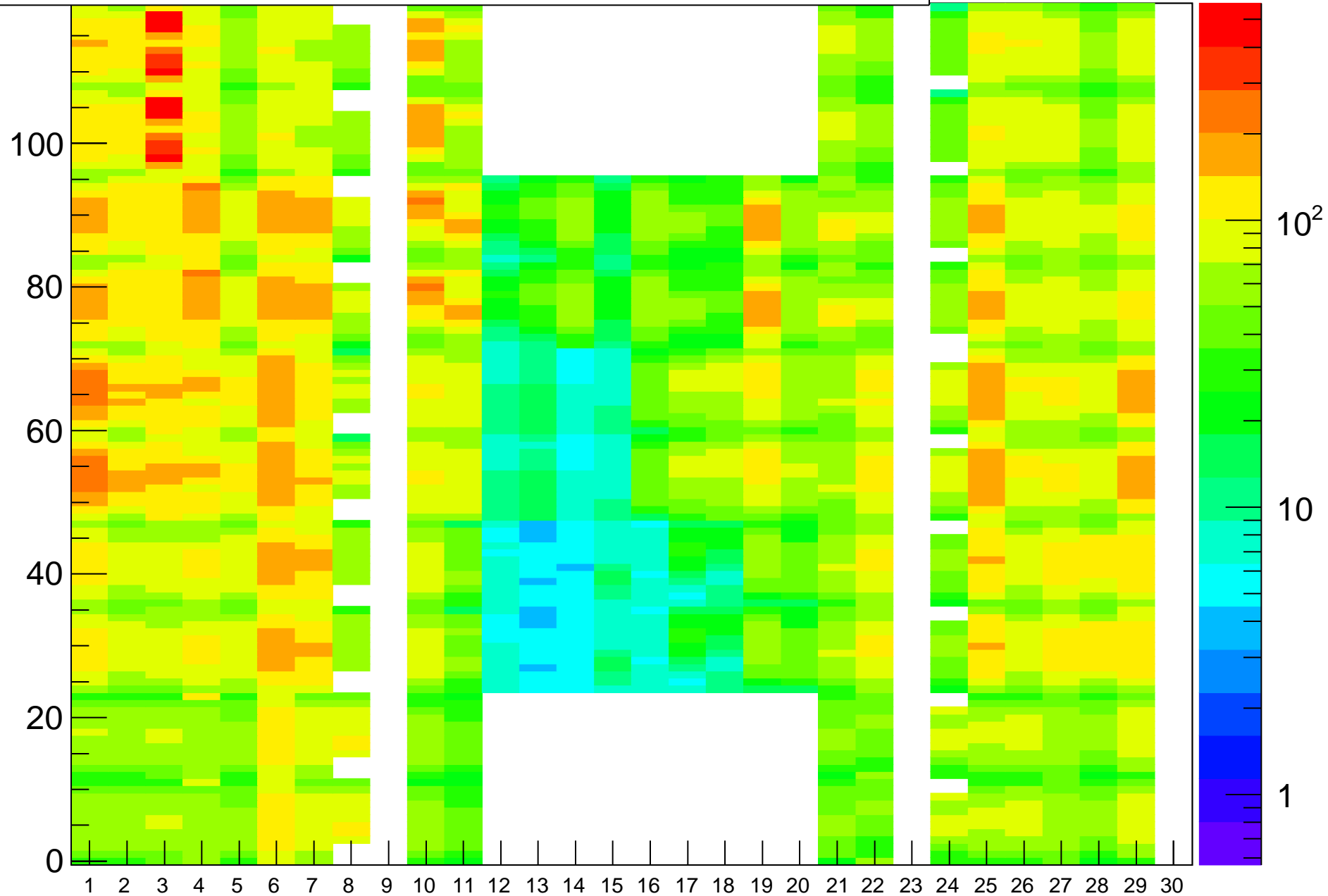
Rate (Hz) vs (BL,strip-posn), Run=19063
