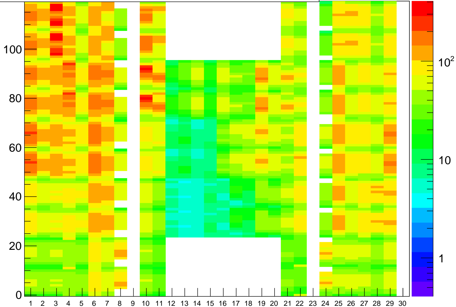
Rate (Hz) vs (BL,strip-posn), Run=19065
