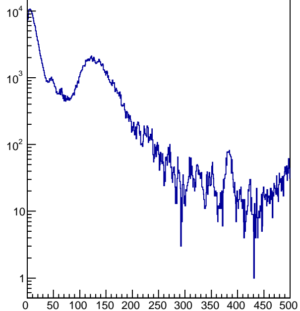
t-t_{\text{ear}}, n\text{Hits}/\text{tray}/\text{ev}>25
