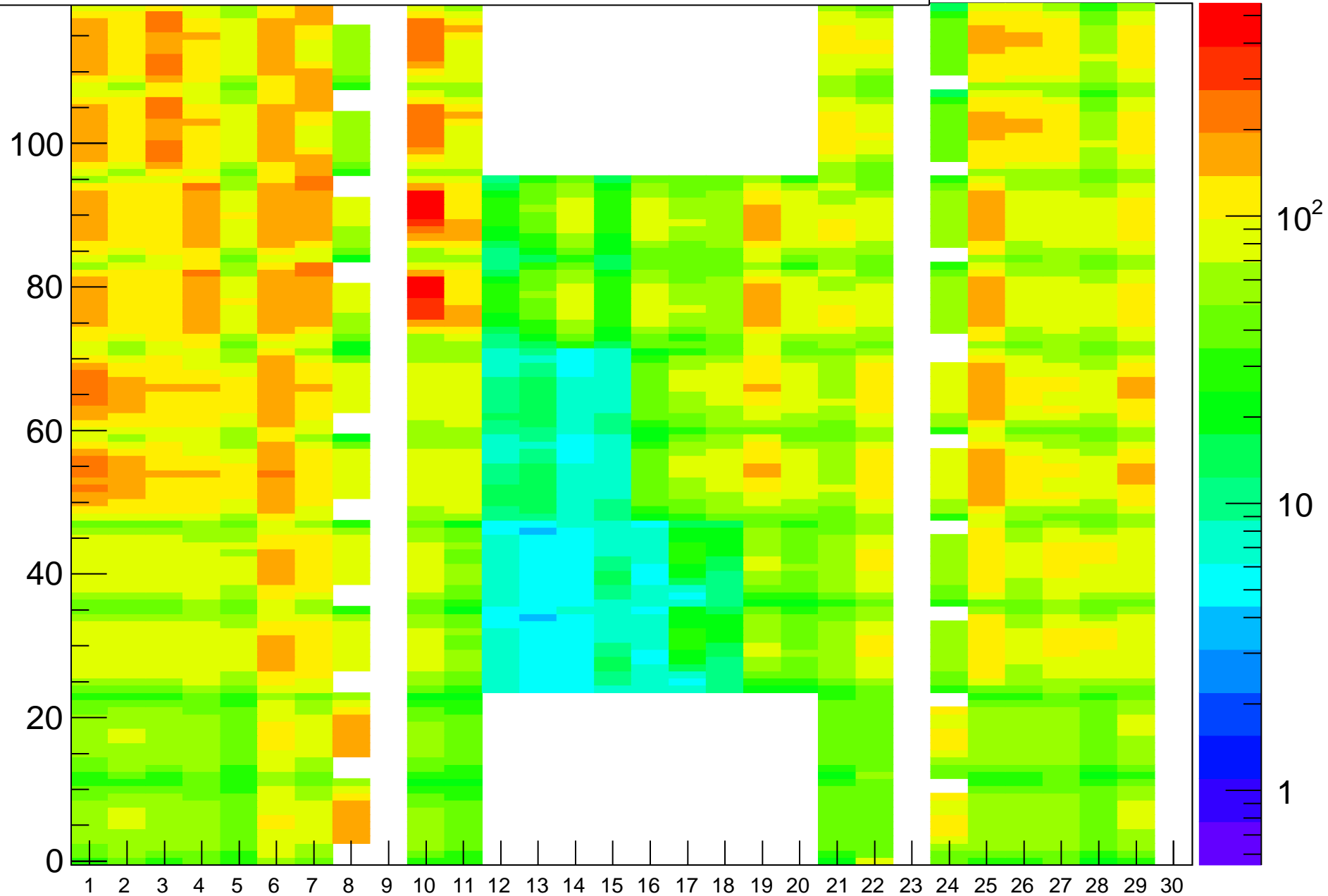
Rate (Hz) vs (BL,strip-posn), Run=19071
