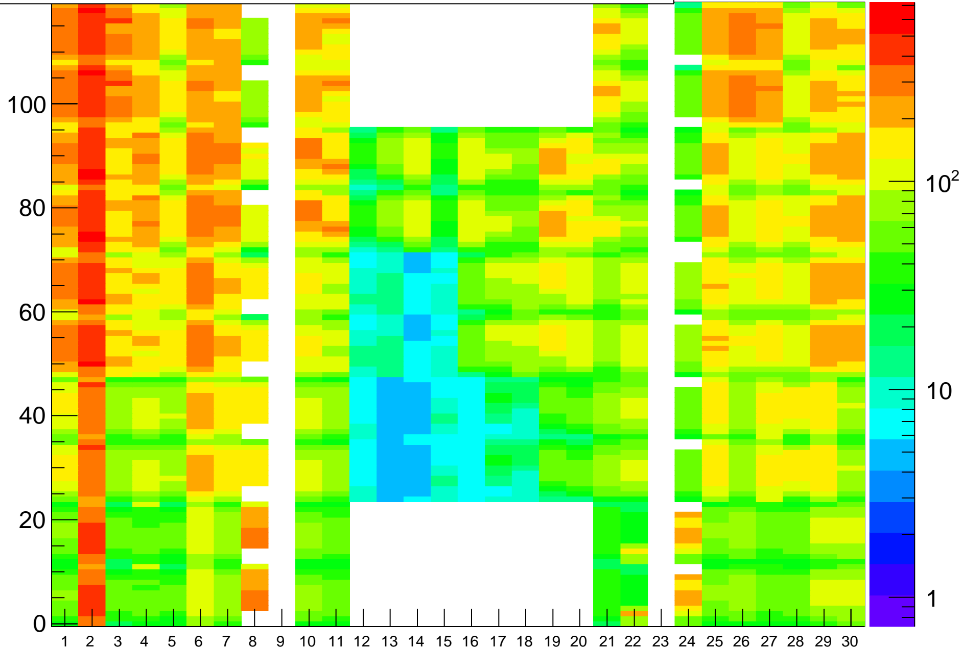
Rate (Hz) vs (BL,strip-posn), Run=19098
