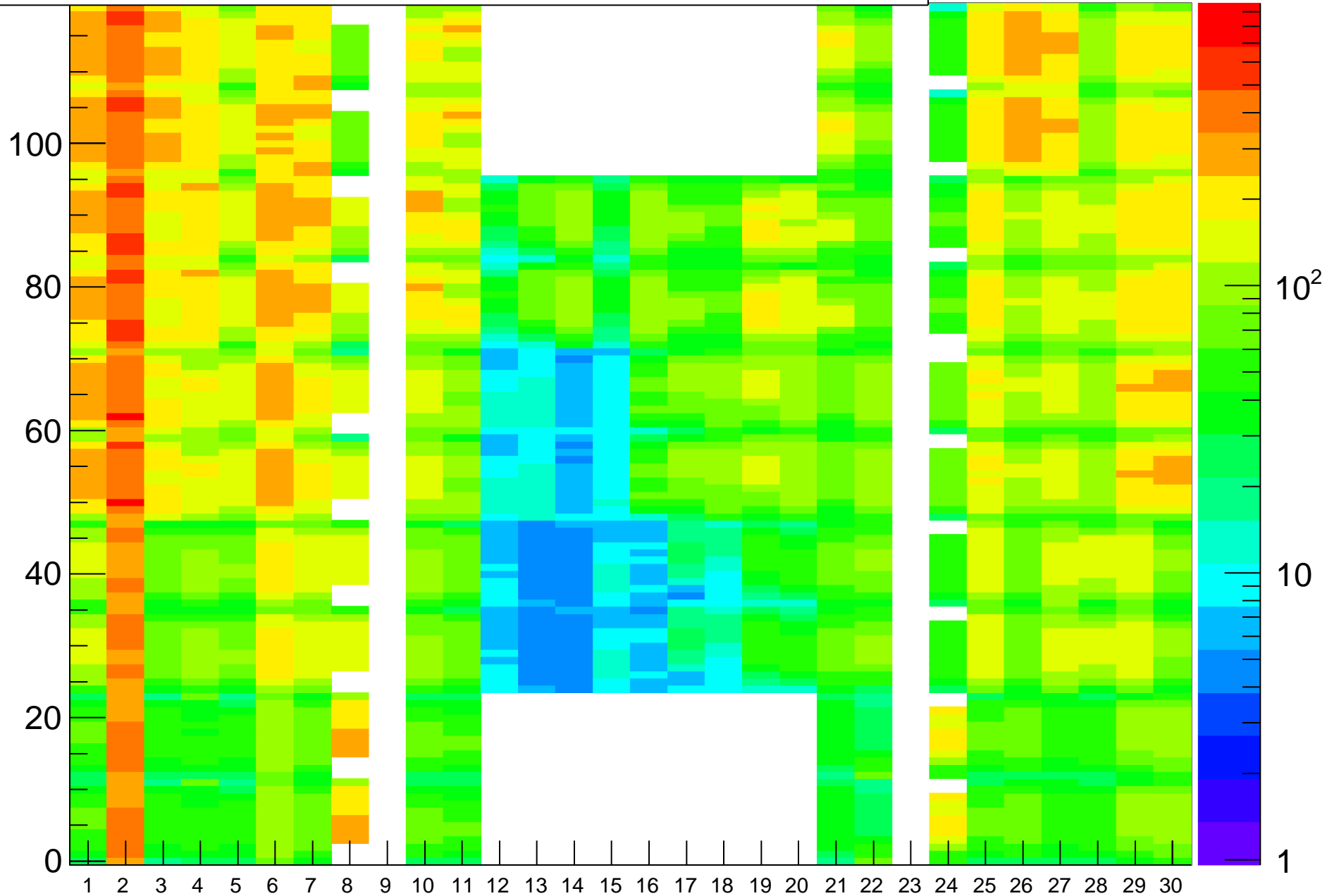
Rate (Hz) vs (BL,strip-posn), Run=19100
