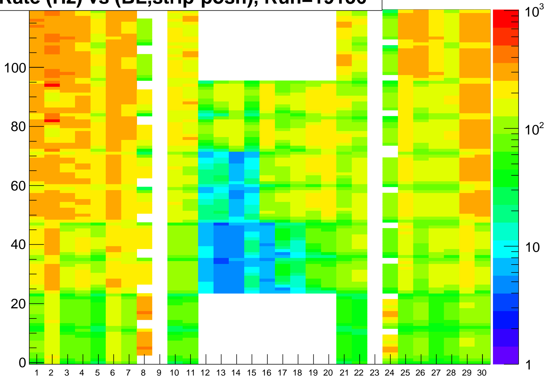
Rate (Hz) vs (BL,strip-posn), Run=19136
