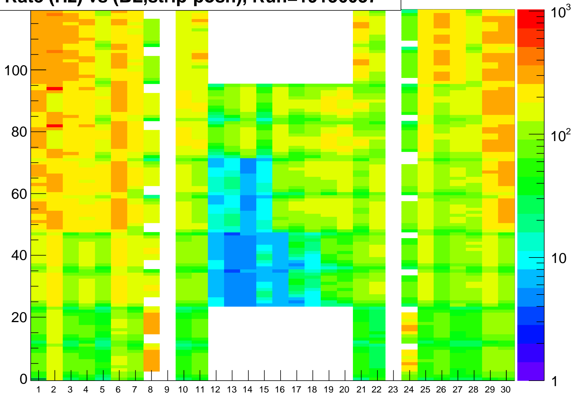
Rate (Hz) vs (BL,strip-posn), Run=19136037
