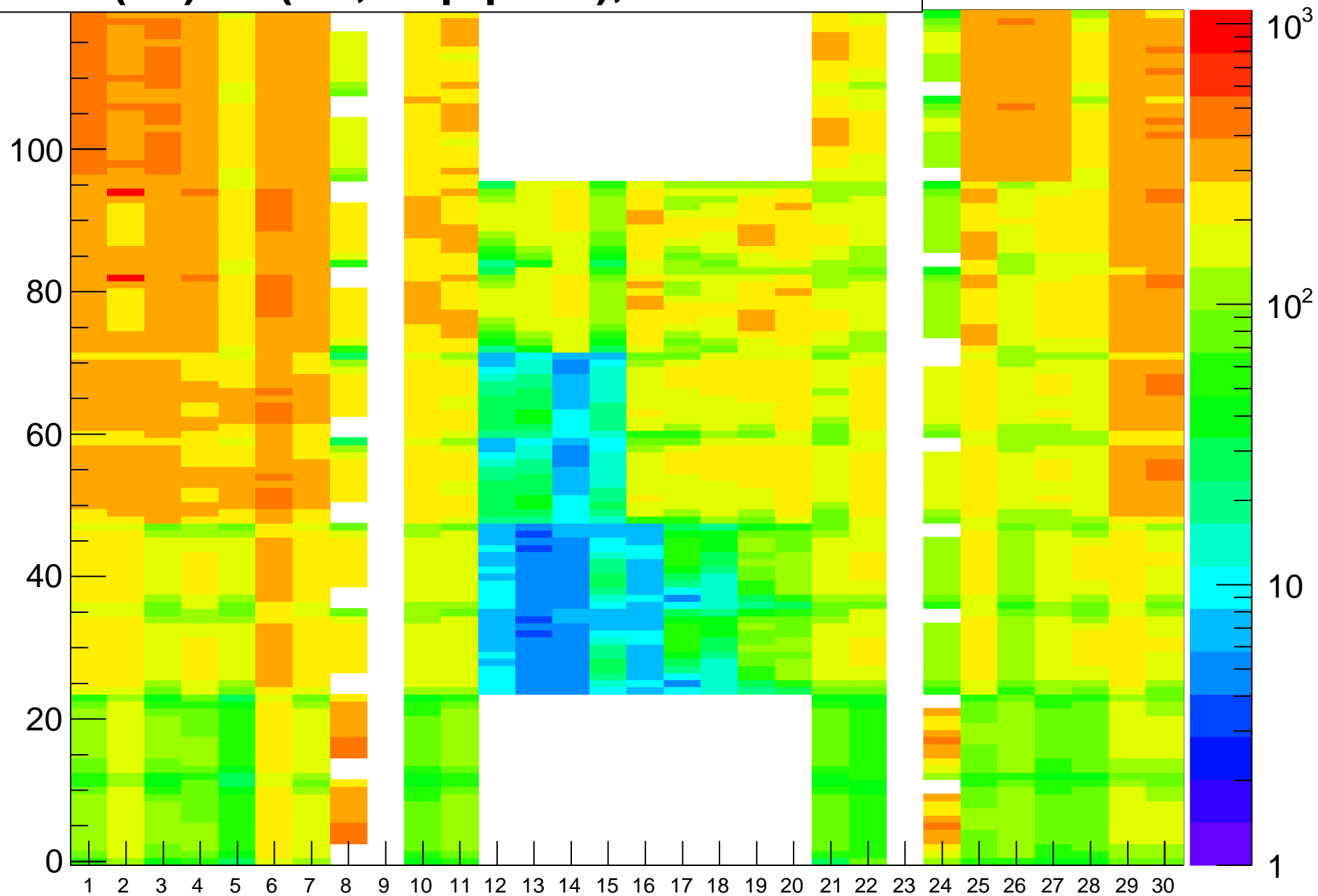
Rate (Hz) vs (BL,strip-posn), Run=19154
