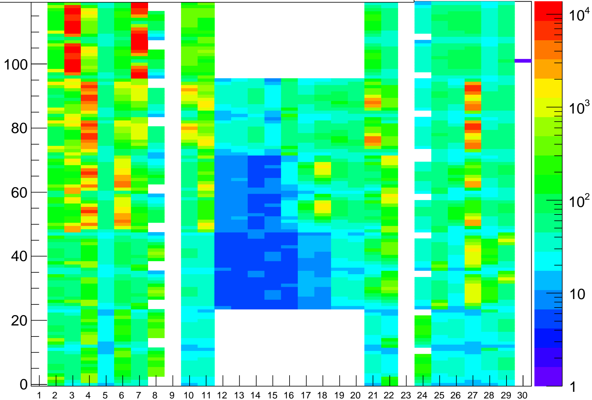
Rate (Hz) vs (BL,strip-posn), Run=20020
