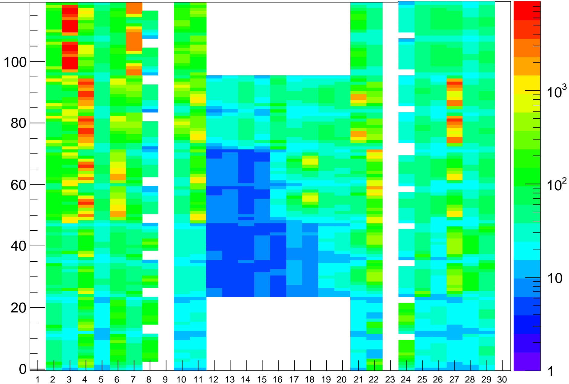
Rate (Hz) vs (BL,strip-posn), Run=20025
