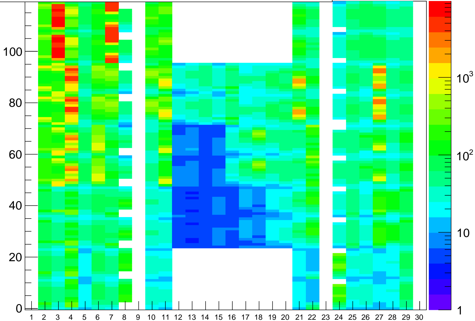
Rate (Hz) vs (BL,strip-posn), Run=20037
