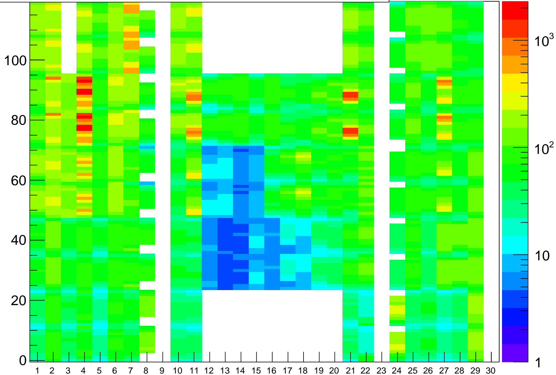
Rate (Hz) vs (BL,strip-posn), Run=20071
