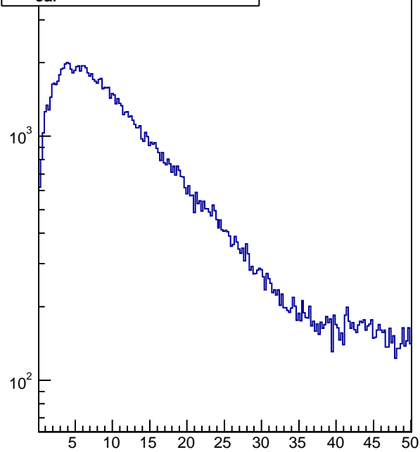
t-t_{\text{ear}}, n\text{Hits}/\text{tray}/\text{ev}>25
