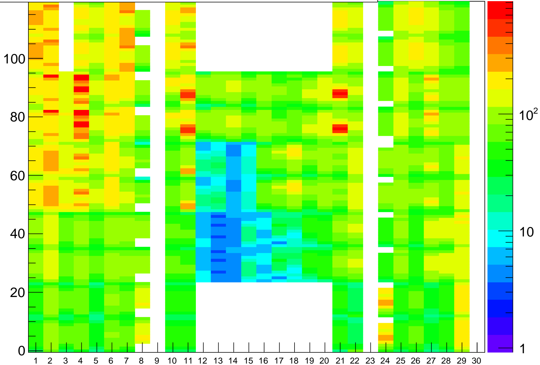
Rate (Hz) vs (BL,strip-posn), Run=20088
