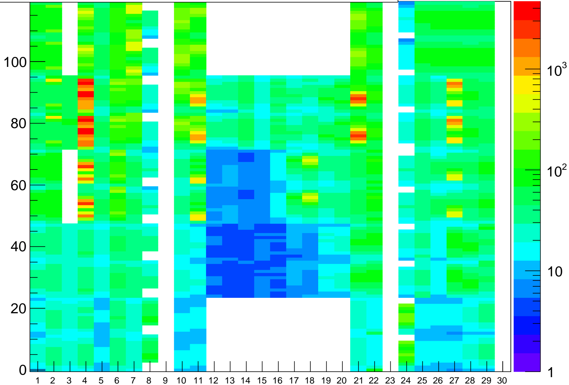
Rate (Hz) vs (BL,strip-posn), Run=20336
