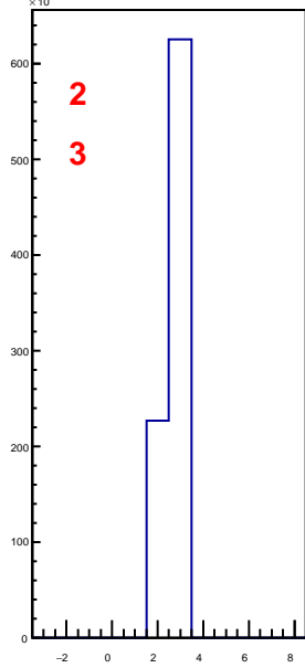
hbunchidoffset_thubhalf00
