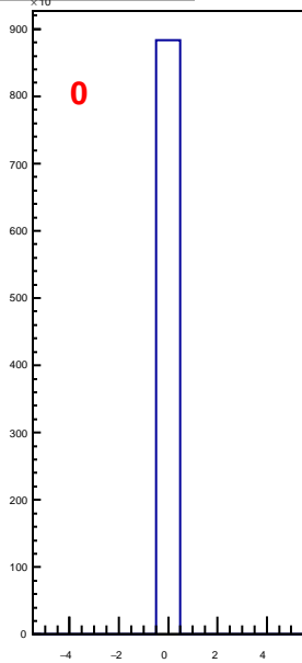
hbunchidoffset_thubhalf21
