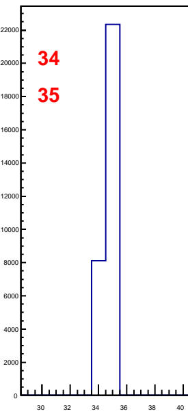
hbunchidoffset_thubhalf40
