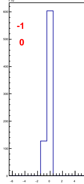
hbunchidoffset_thubhalf30
