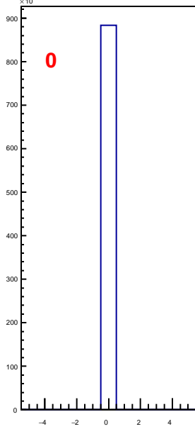
hbunchidoffset_thubhalf20
