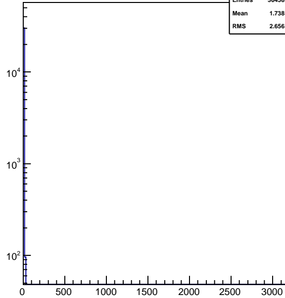
hhhitstof_xingm7_vpd
