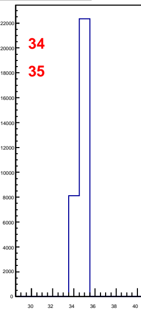
hbunchidoffset_thubhalf41
