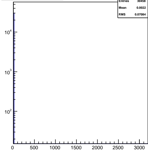
hnhitstof_xingp7
