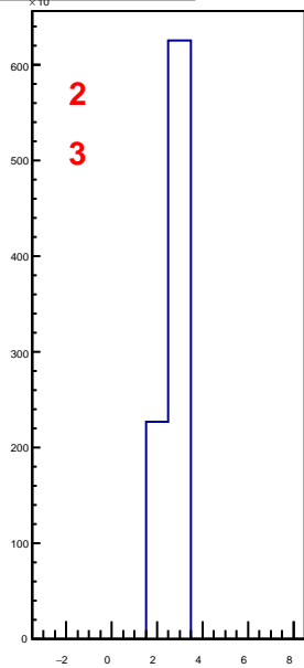
hbunchidoffset_thubhalf01
