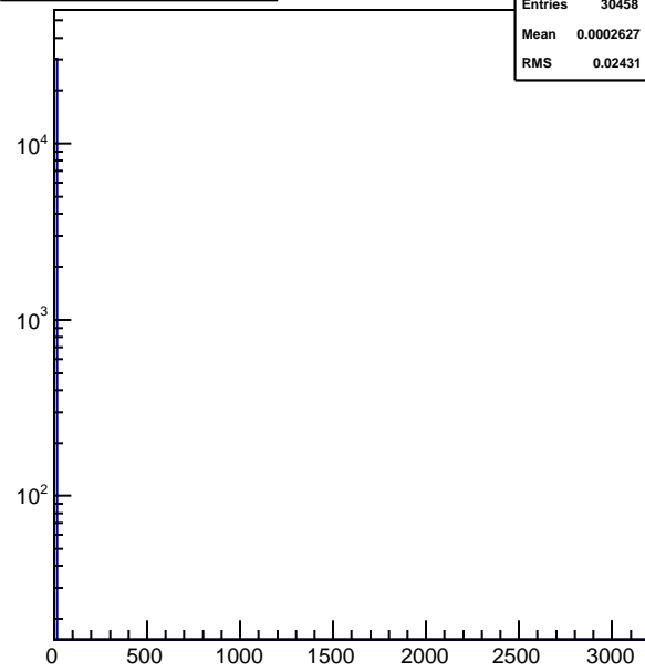
hnhitstof_xingm7
