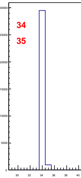
hbunchidoffset_thubhalf50
