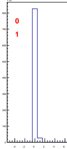
hbunchidoffset_thubhalf10
