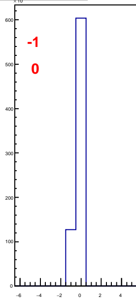
hbunchidoffset_thubhalf31
