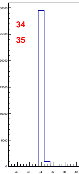
hbunchidoffset_thubhalf51
