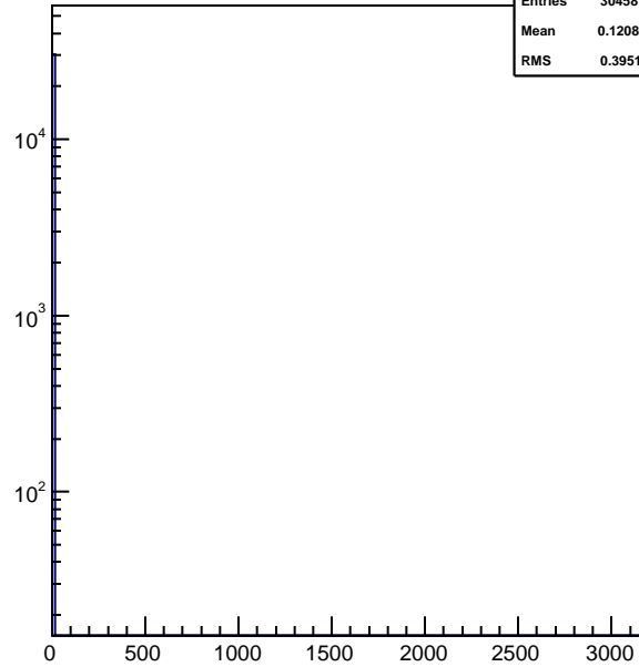
hhhitstof_xingm7_vpd
