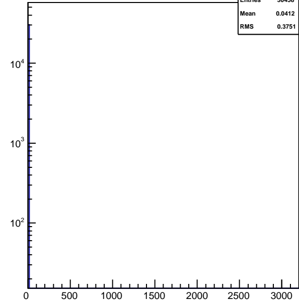
hhhitstof_xingp7_vpd
