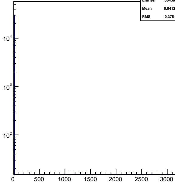
hhhitstof_xingp2_vpd
