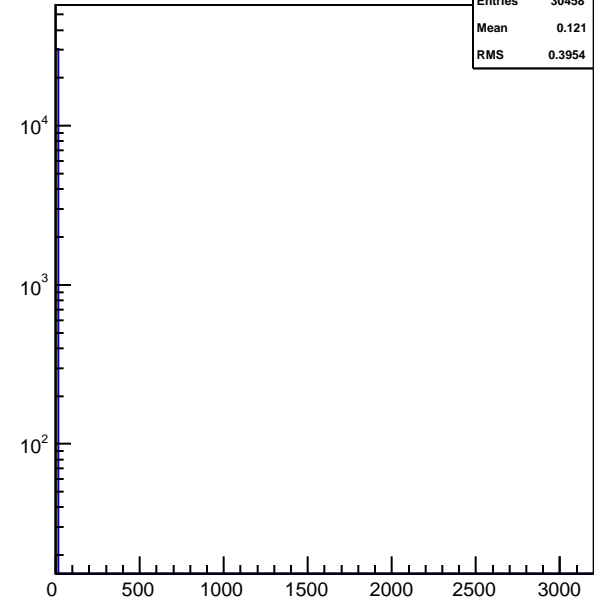
hhhitstof_xingp7_vpd
