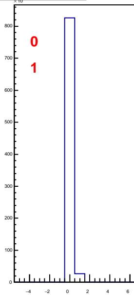
hbunchidoffset_thubhalf11
