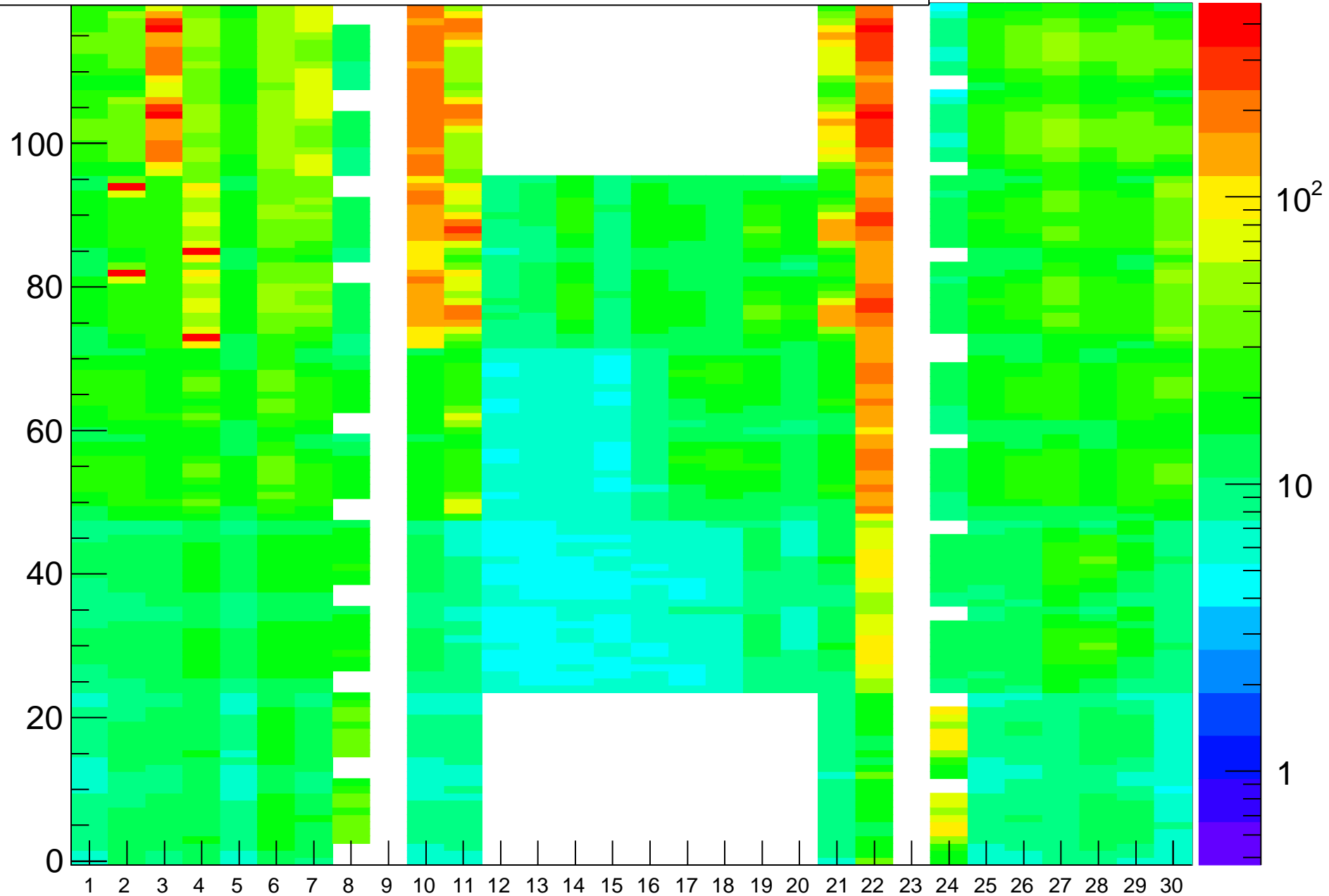
Rate (Hz) vs (BL,strip-posn), Run=22335
