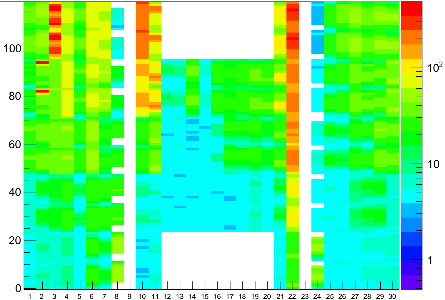
Rate (Hz) vs (BL,strip-posn), Run=22345
