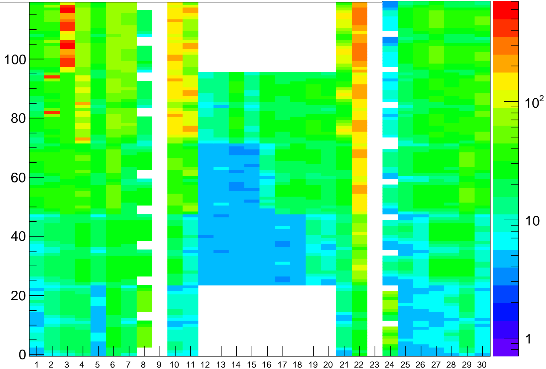
Rate (Hz) vs (BL,strip-posn), Run=22353
