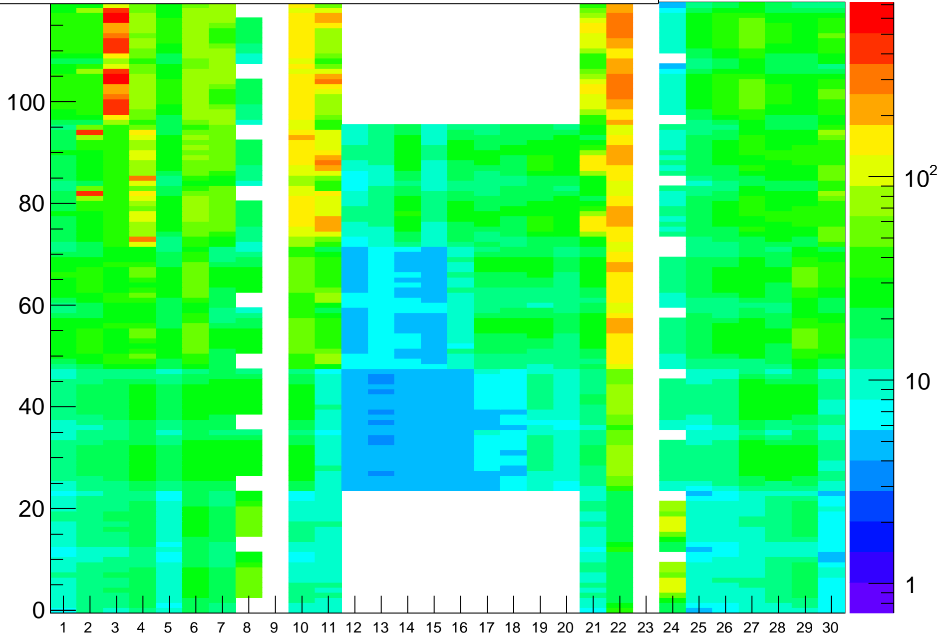
Rate (Hz) vs (BL,strip-posn), Run=22354
