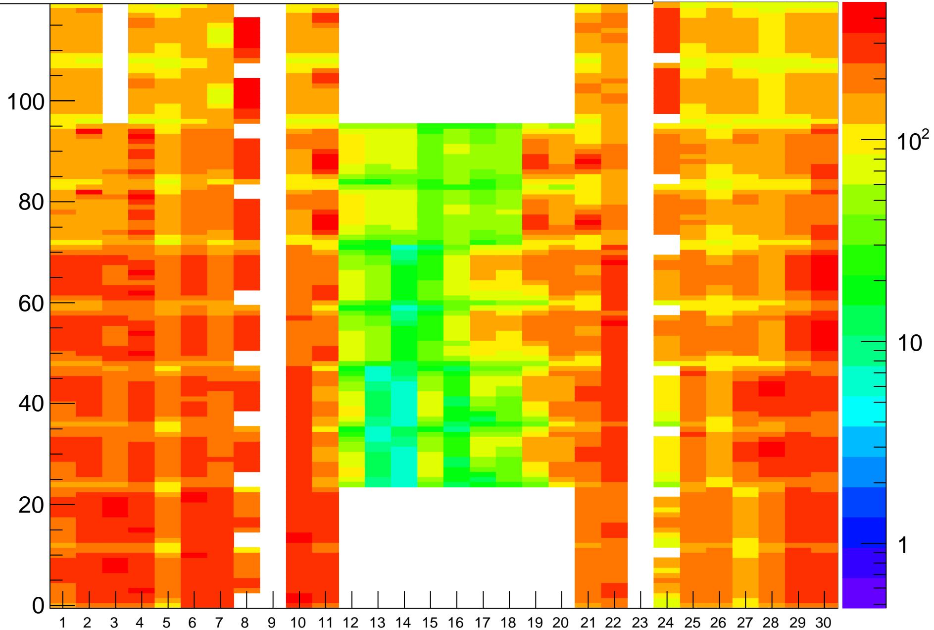
Rate (Hz) vs (BL,strip-posn), Run=23068
