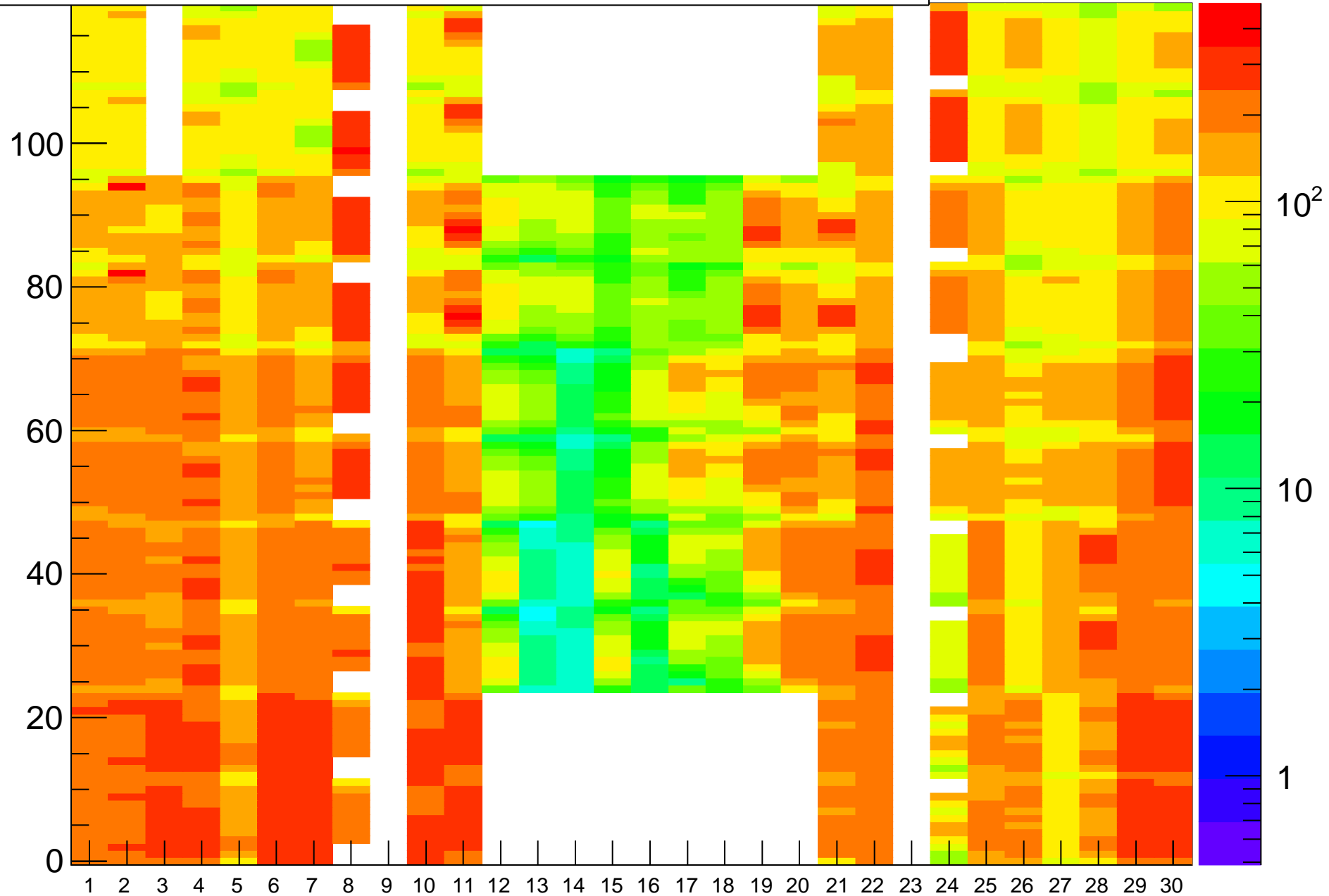
Rate (Hz) vs (BL,strip-posn), Run=23077
