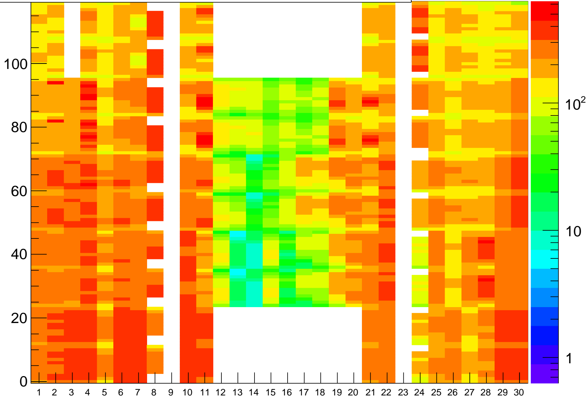
Rate (Hz) vs (BL,strip-posn), Run=23078
