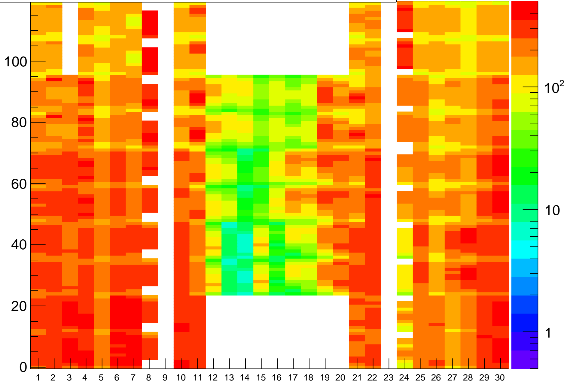
Rate (Hz) vs (BL,strip-posn), Run=23081
