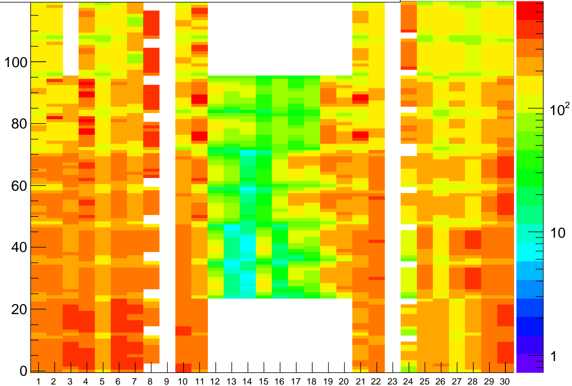
Rate (Hz) vs (BL,strip-posn), Run=23084
