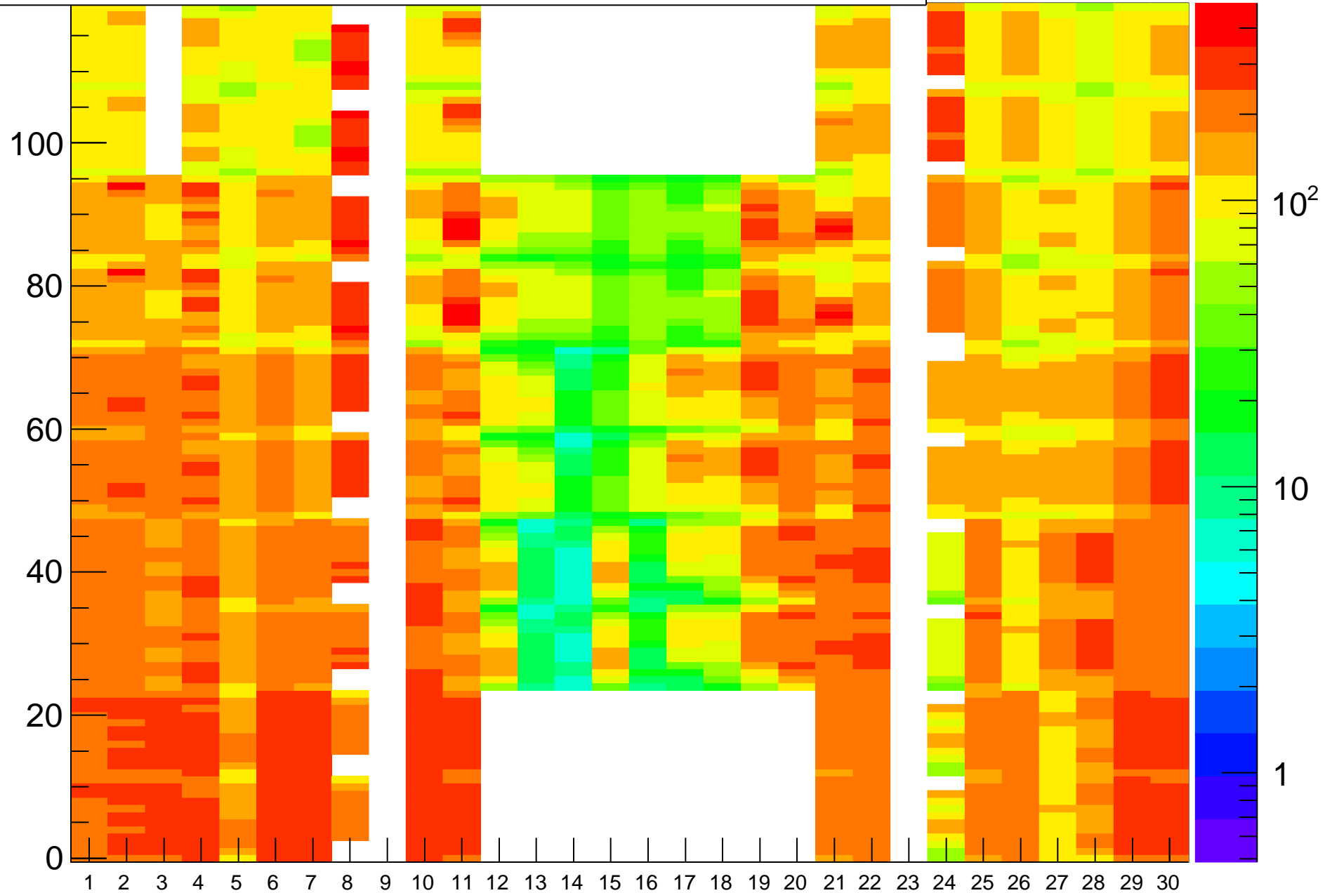
Rate (Hz) vs (BL,strip-posn), Run=23095
