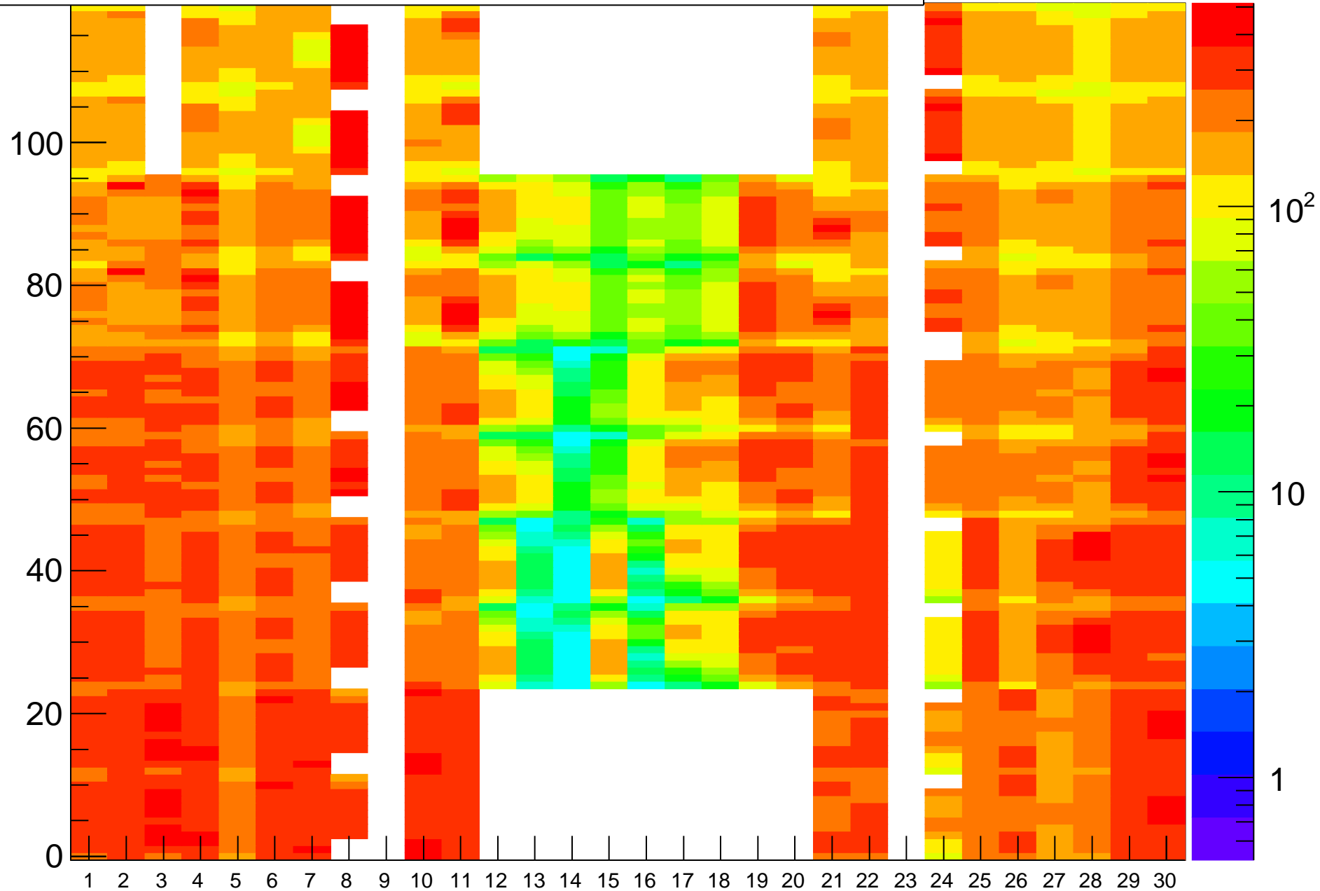
Rate (Hz) vs (BL,strip-posn), Run=23096
