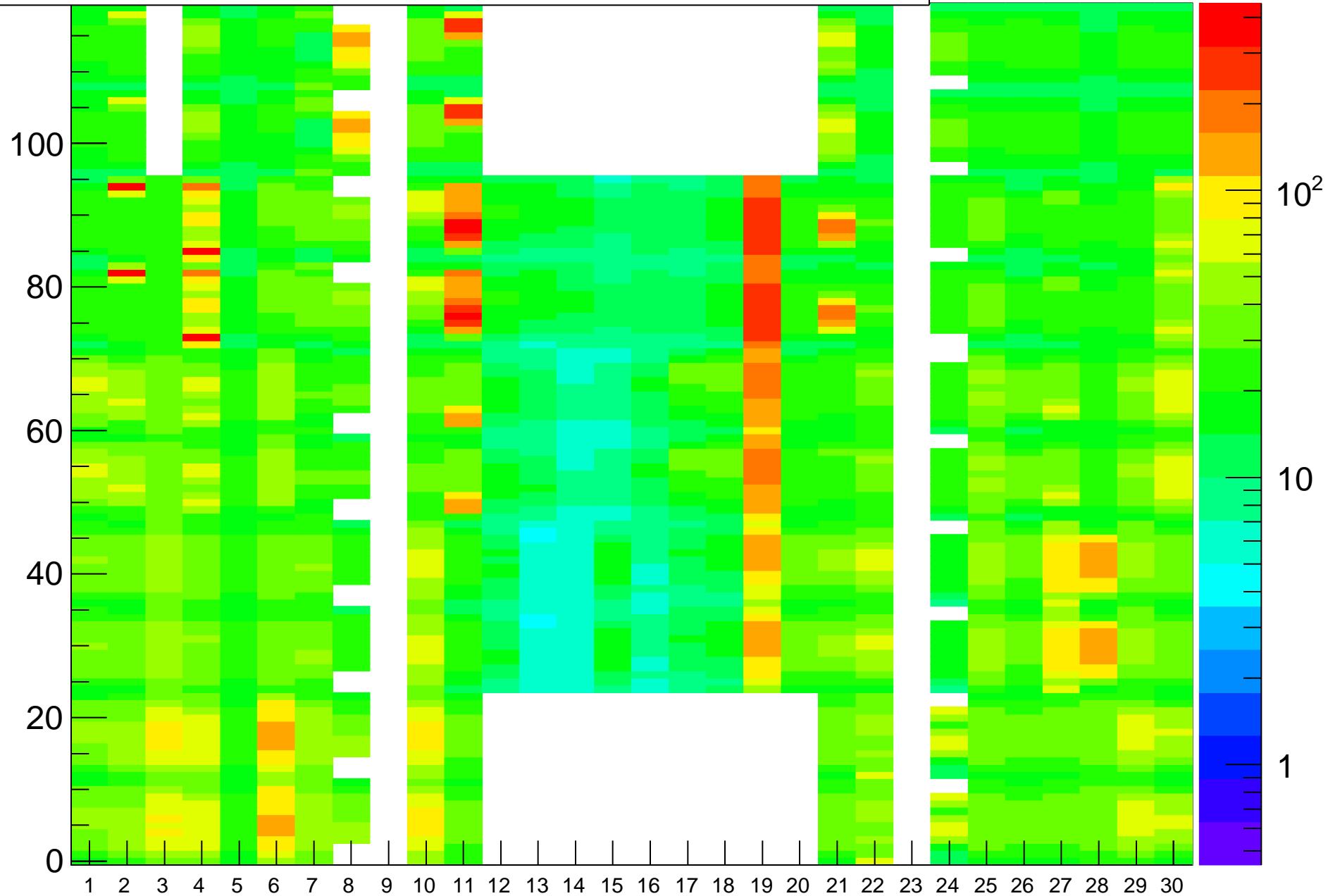
Rate (Hz) vs (BL,strip-posn), Run=24119
