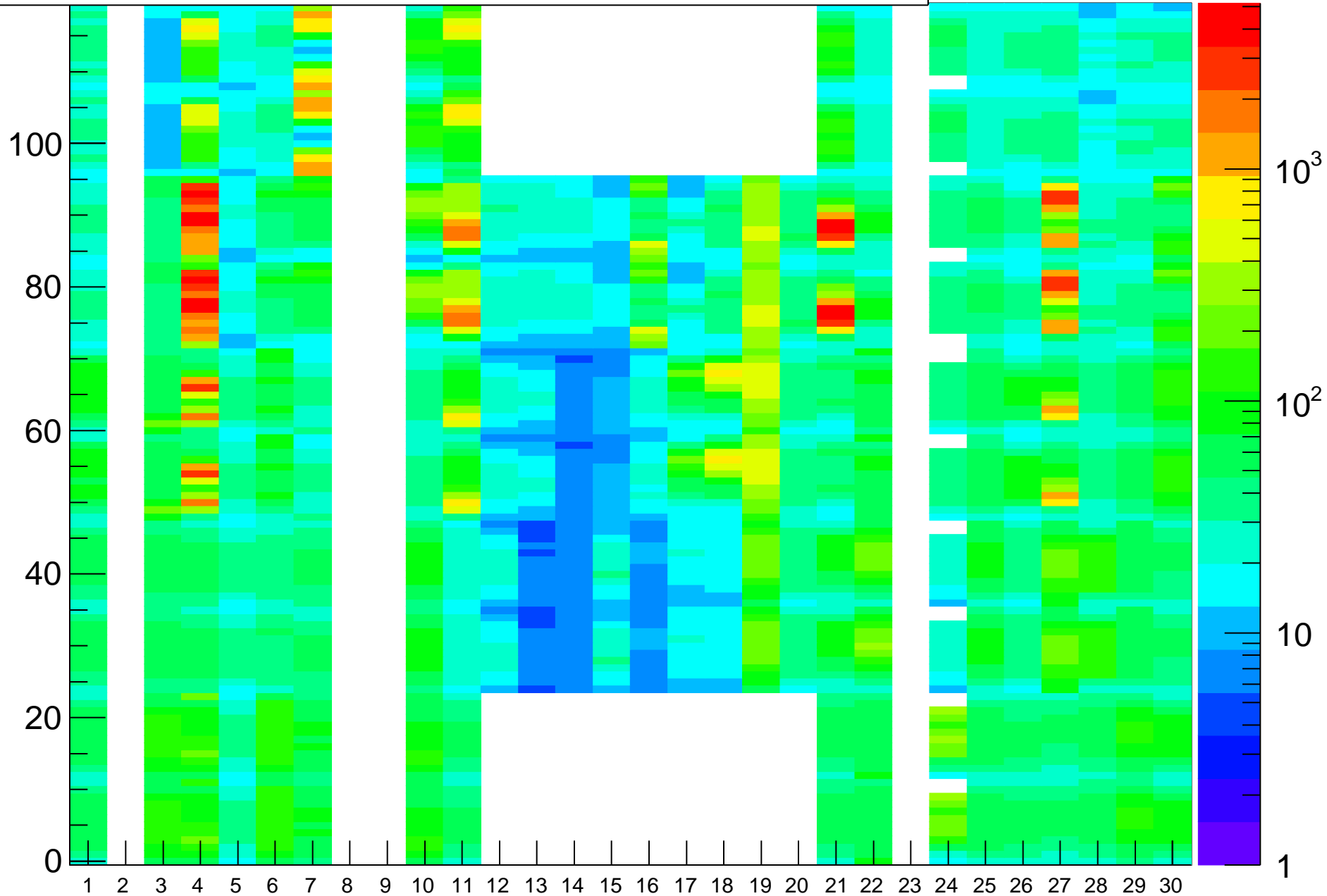
Rate (Hz) vs (BL,strip-posn), Run=24137
