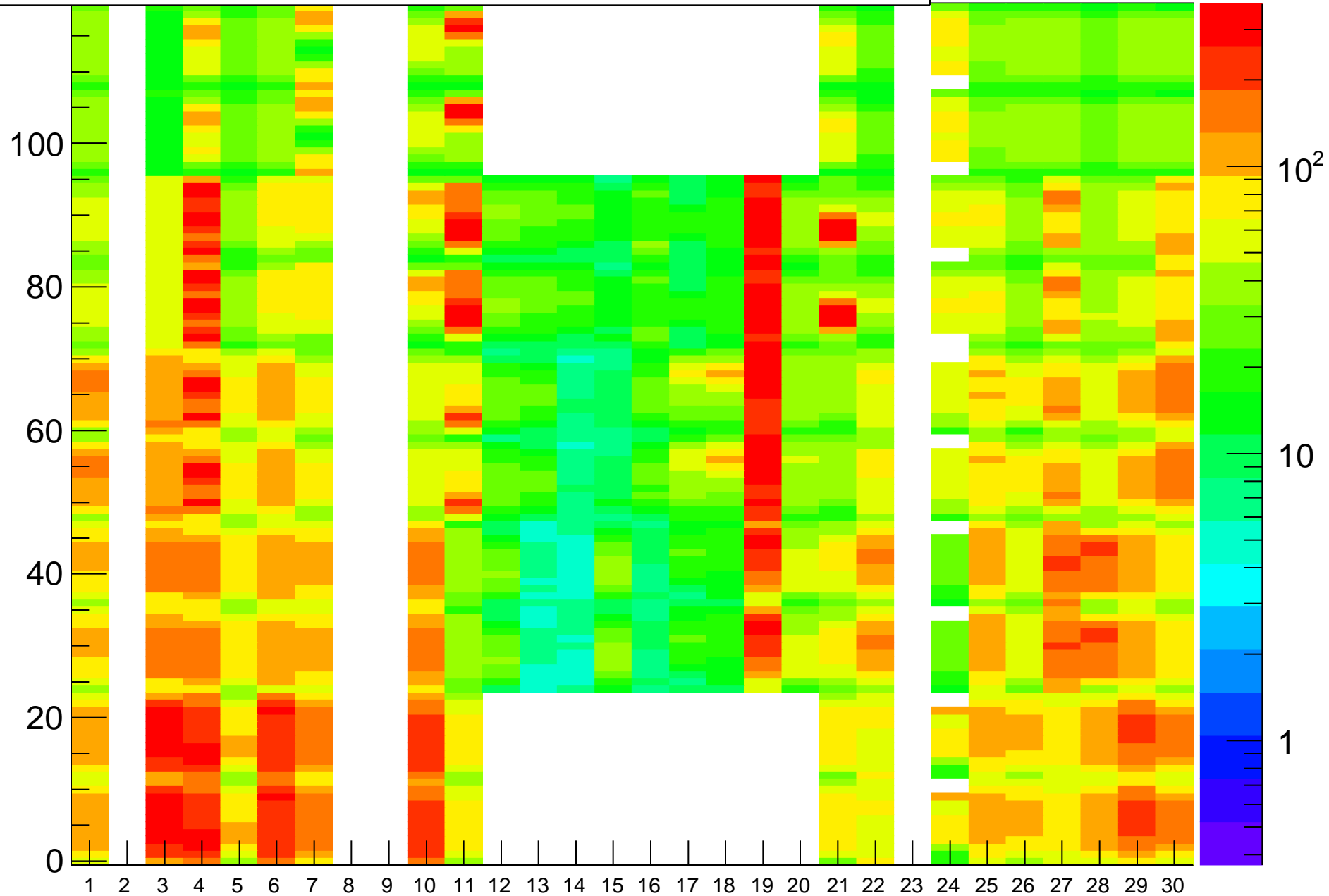
Rate (Hz) vs (BL,strip-posn), Run=24150
