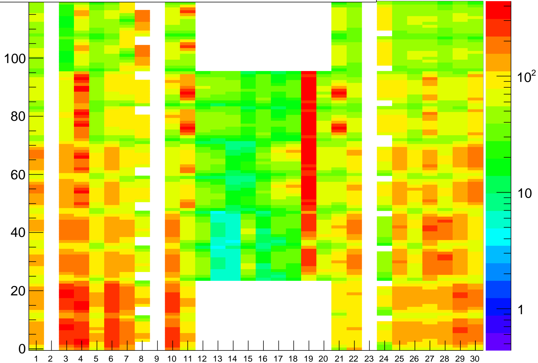
Rate (Hz) vs (BL,strip-posn), Run=24153
