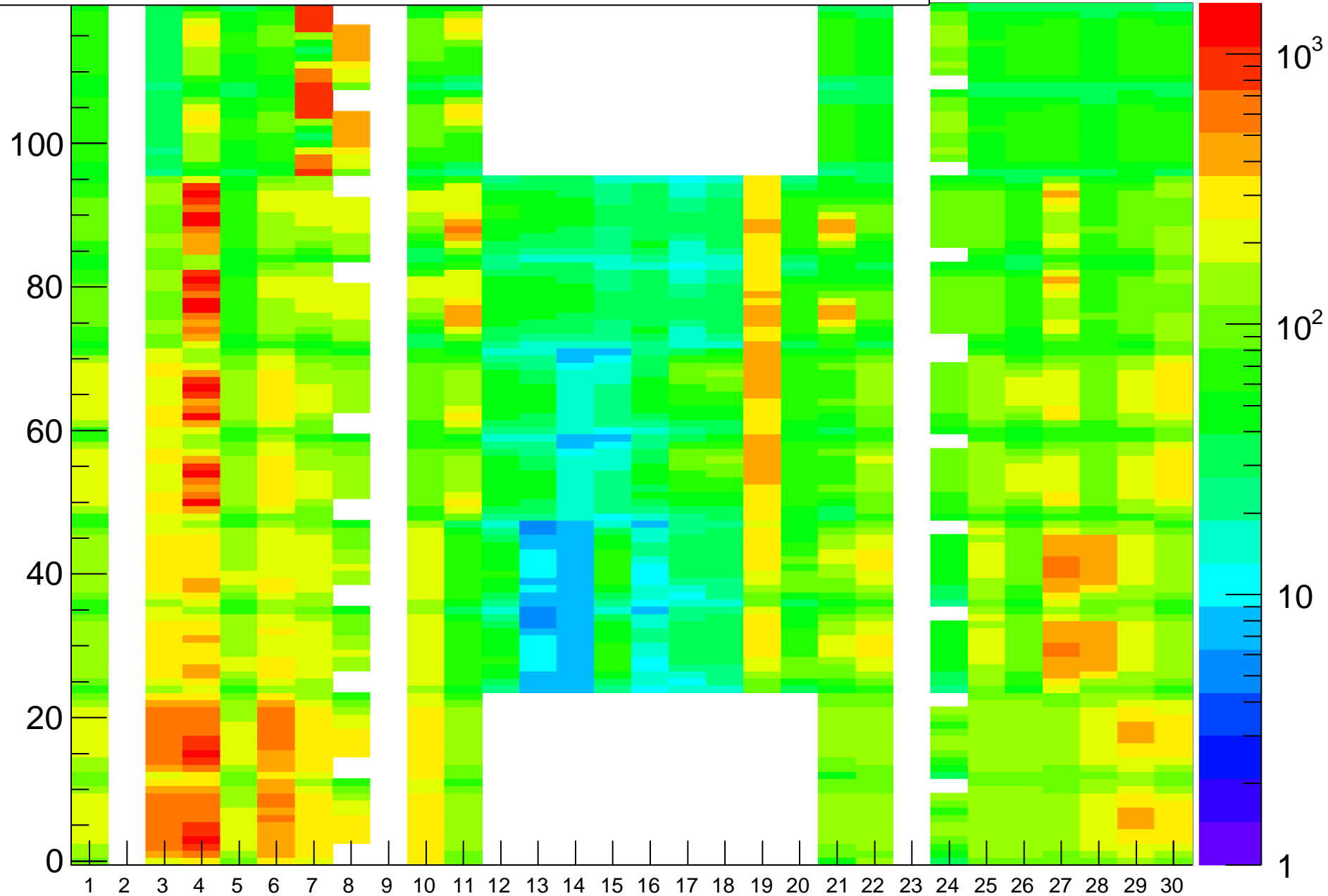
Rate (Hz) vs (BL,strip-posn), Run=24161
