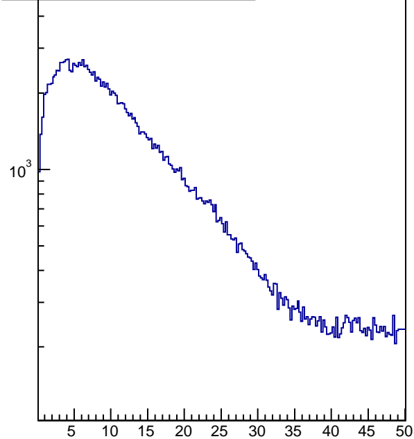
t-t_{\text{ear}}, n\text{Hits}/\text{tray}/\text{ev}>25
