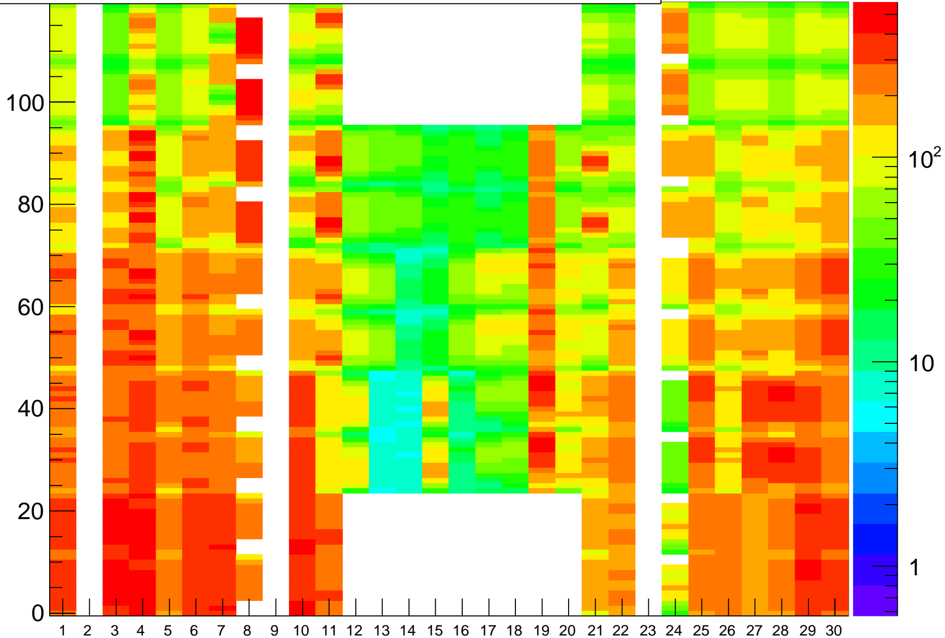
Rate (Hz) vs (BL,strip-posn), Run=24184
