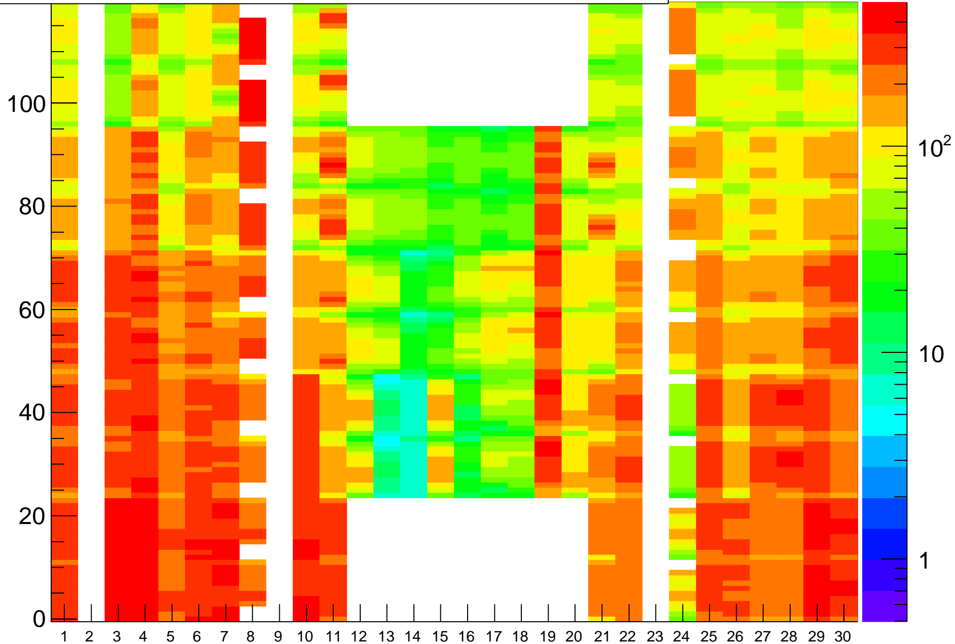
Rate (Hz) vs (BL,strip-posn), Run=24186
