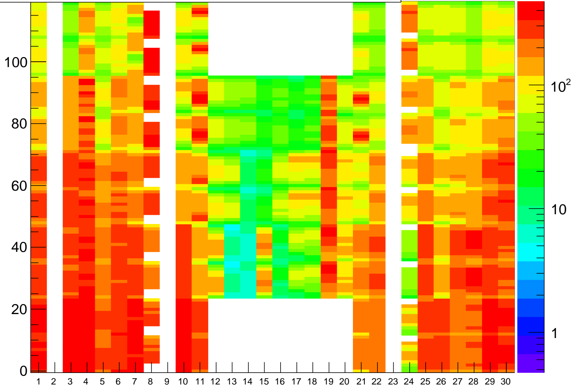
Rate (Hz) vs (BL,strip-posn), Run=24188
