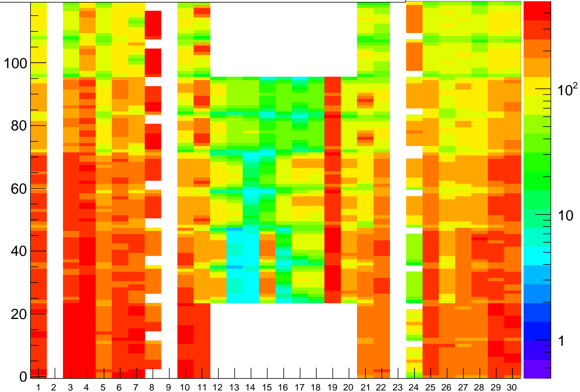
Rate (Hz) vs (BL,strip-posn), Run=24193
