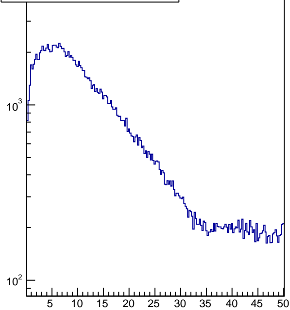
t-t_{\text{ear}}, n\text{Hits}/\text{tray}/\text{ev}>25
