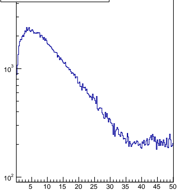
t-t_{\text{ear}} , nHits/tray/ev>25
