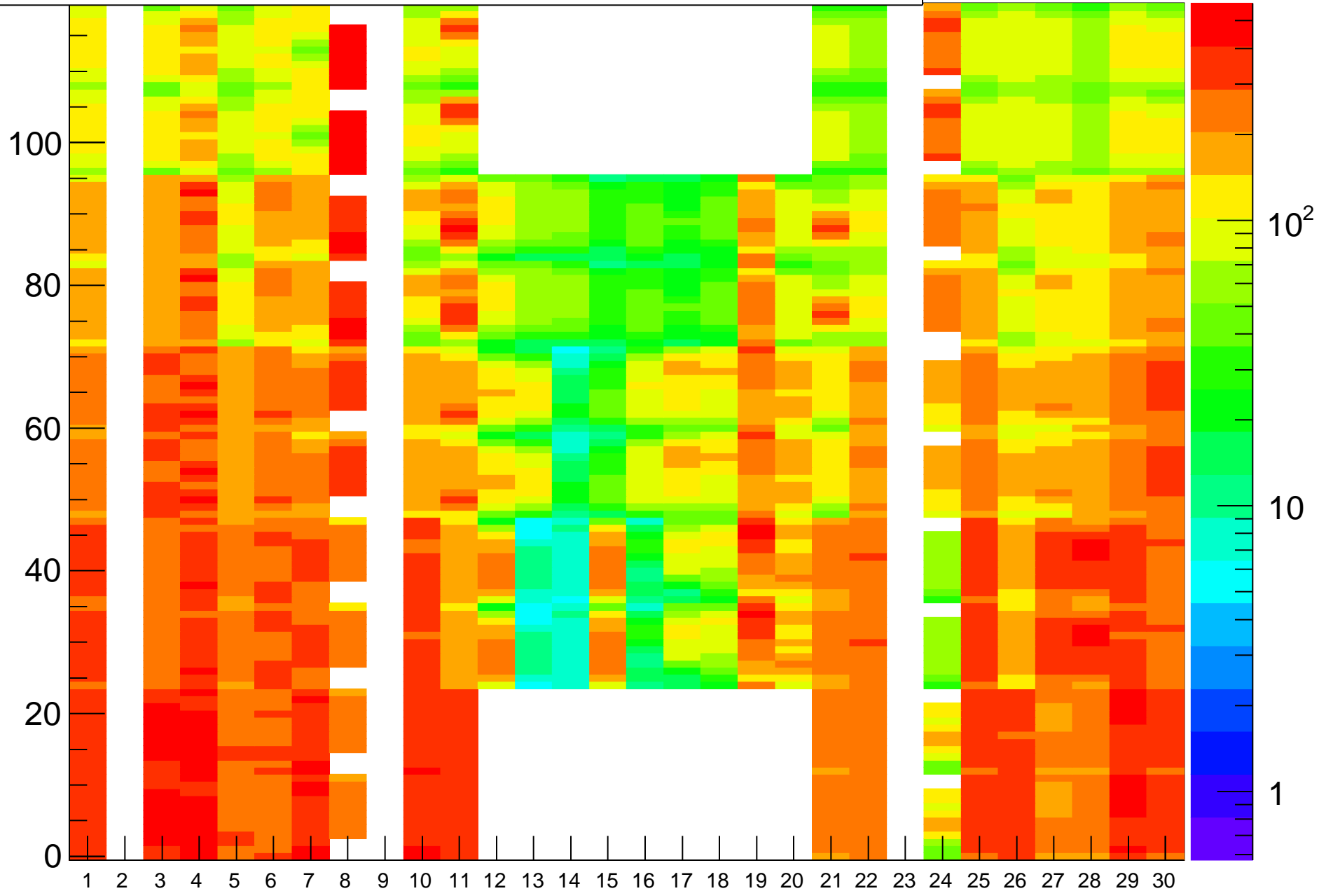
Rate (Hz) vs (BL,strip-posn), Run=24205
