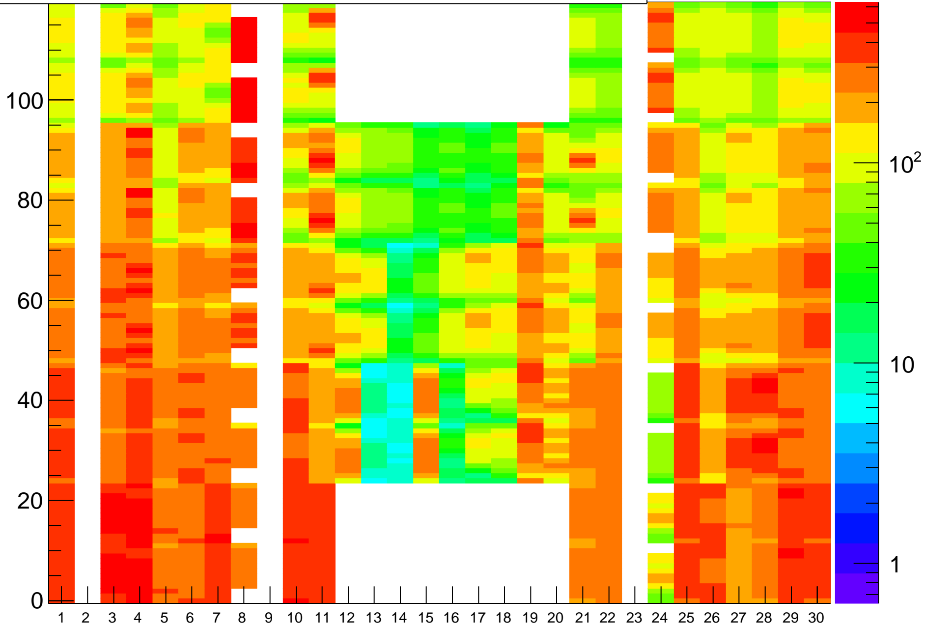
Rate (Hz) vs (BL,strip-posn), Run=24208
