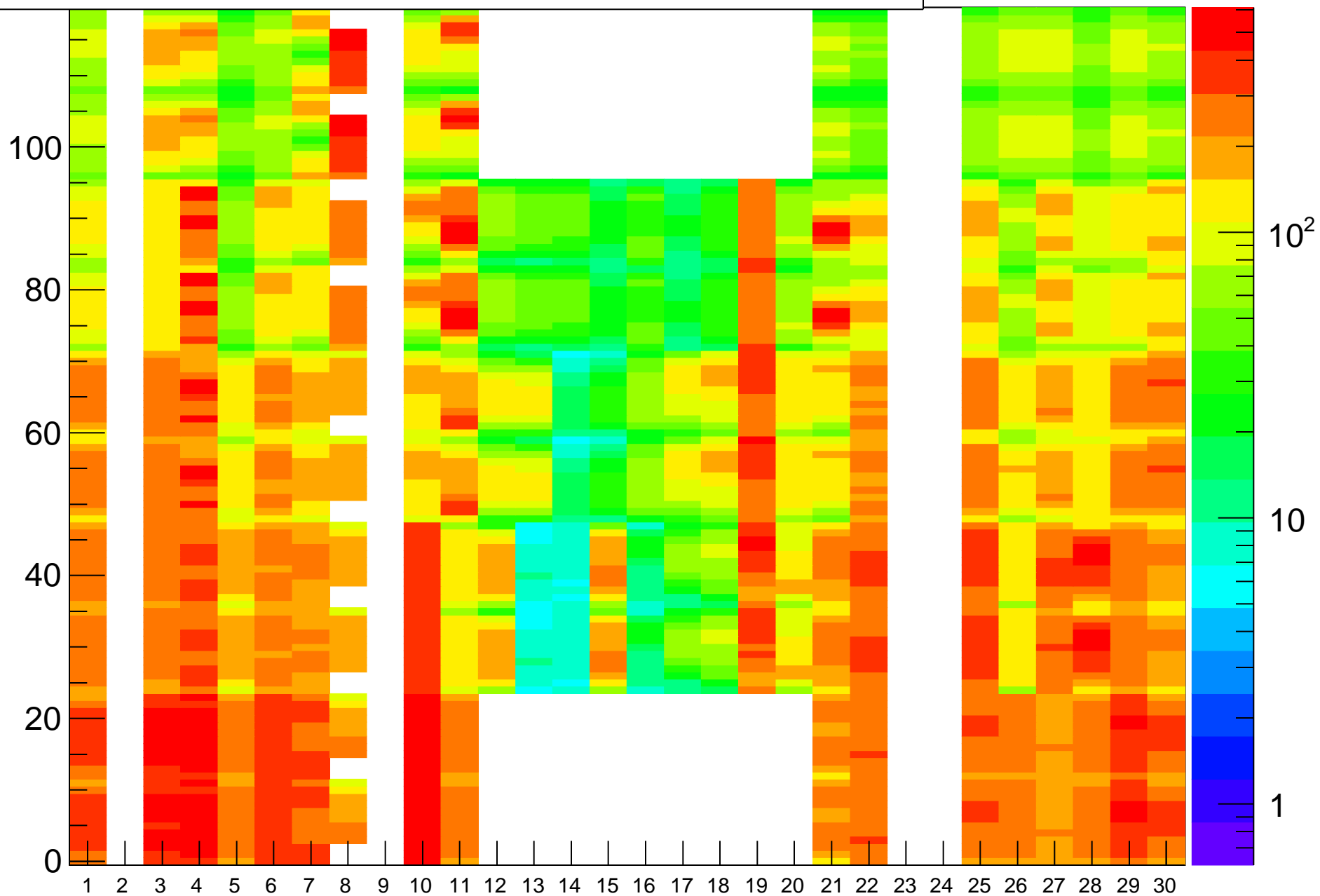
Rate (Hz) vs (BL,strip-posn), Run=25158052
