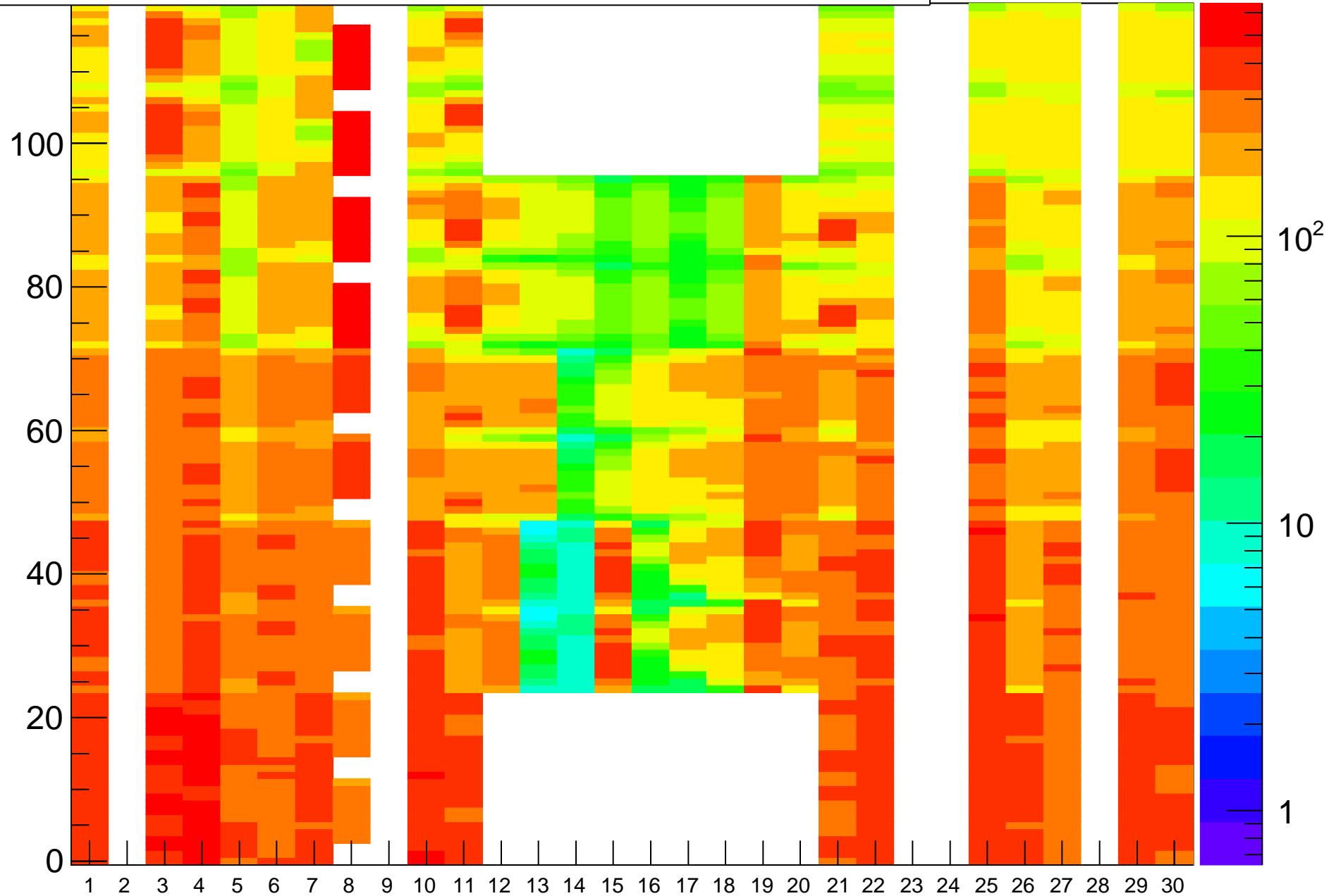
Rate (Hz) vs (BL,strip-posn), Run=25208
