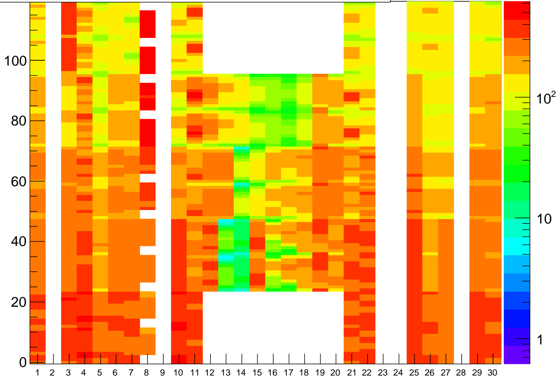
Rate (Hz) vs (BL,strip-posn), Run=25258
