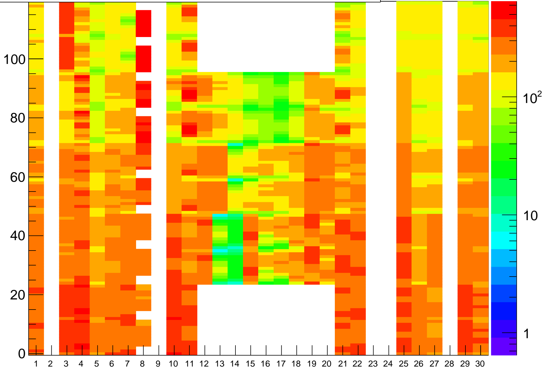
Rate (Hz) vs (BL,strip-posn), Run=25274
