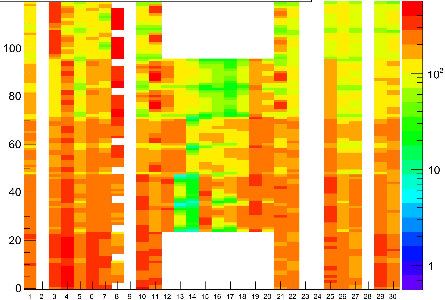
Rate (Hz) vs (BL,strip-posn), Run=25283
