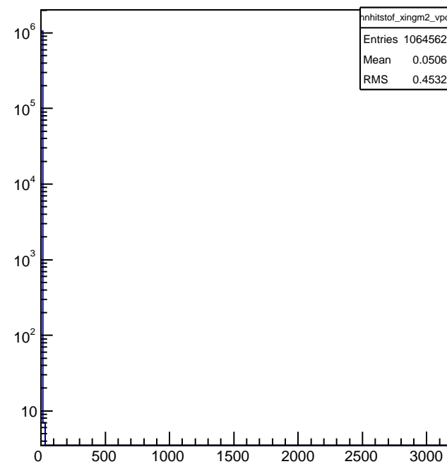
hnhitstof_xingm2_vpd
