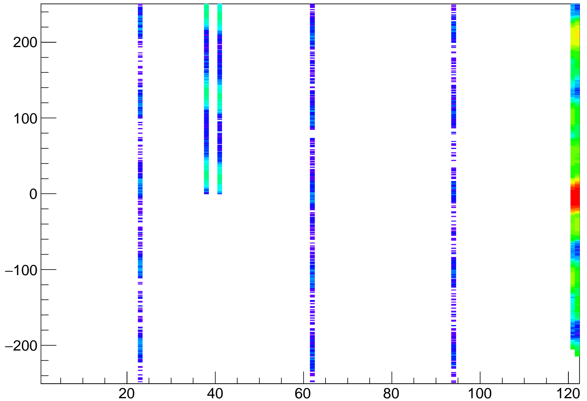
htrgdtime_trayoff
