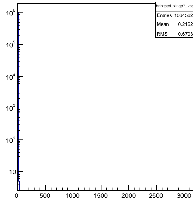
hnhitstof_xingp7_vpd
