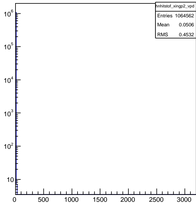
hnhitstof_xingp2_vpd
