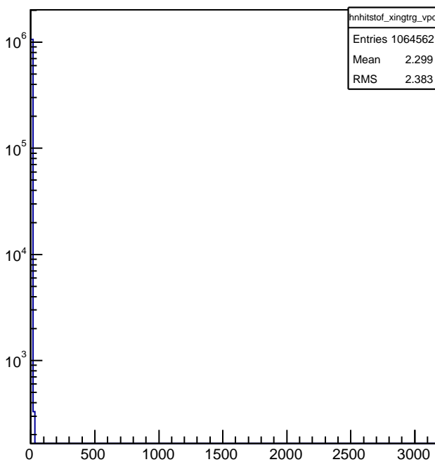
hnhitstof_xingtrg_vpd
