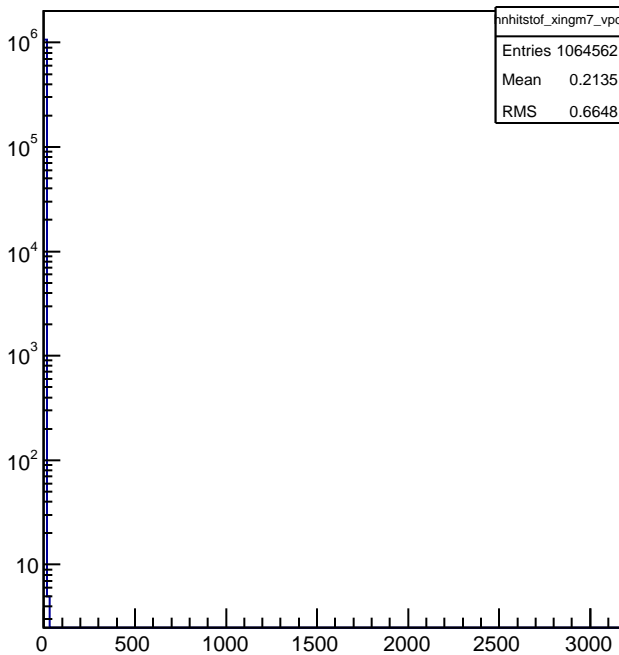
hnhitstof_xingm7_vpd
