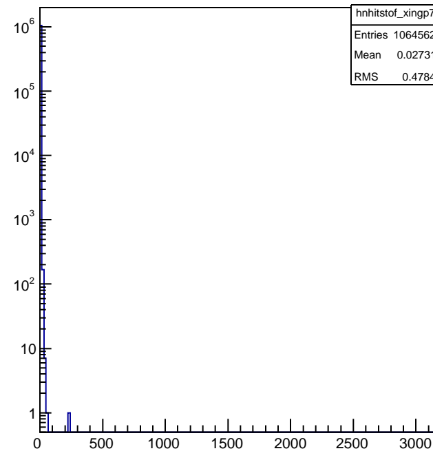
hnhitstof_xingp7
