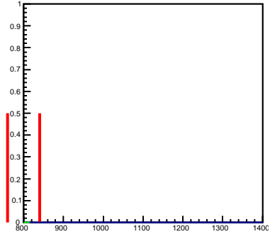
dtrgtime, tray=122
