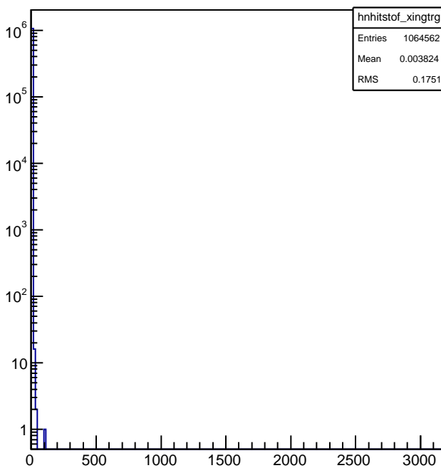
hnhitstof_xingtrg
