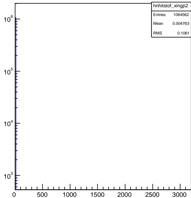
hnhitstof_xingp2
