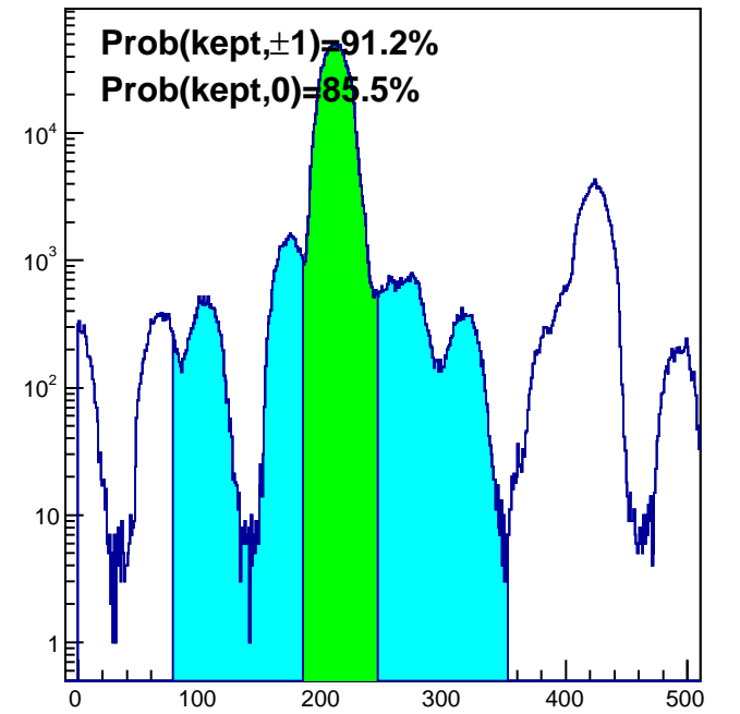
trgdtime, VPD 122
