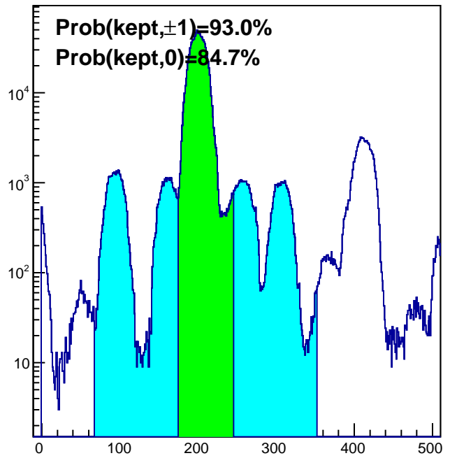
trgdtime, VPD 121
