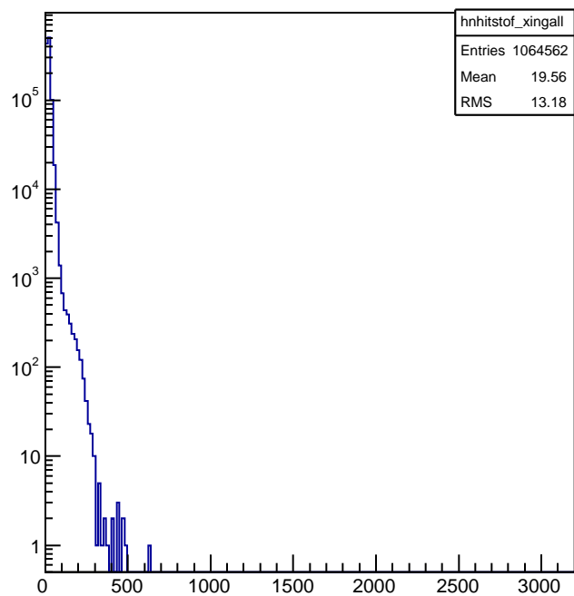
hnhitstof_xingall
