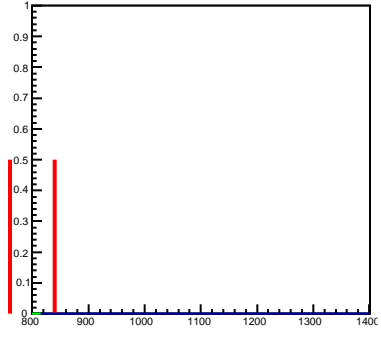
dtrgtime, tray=121
