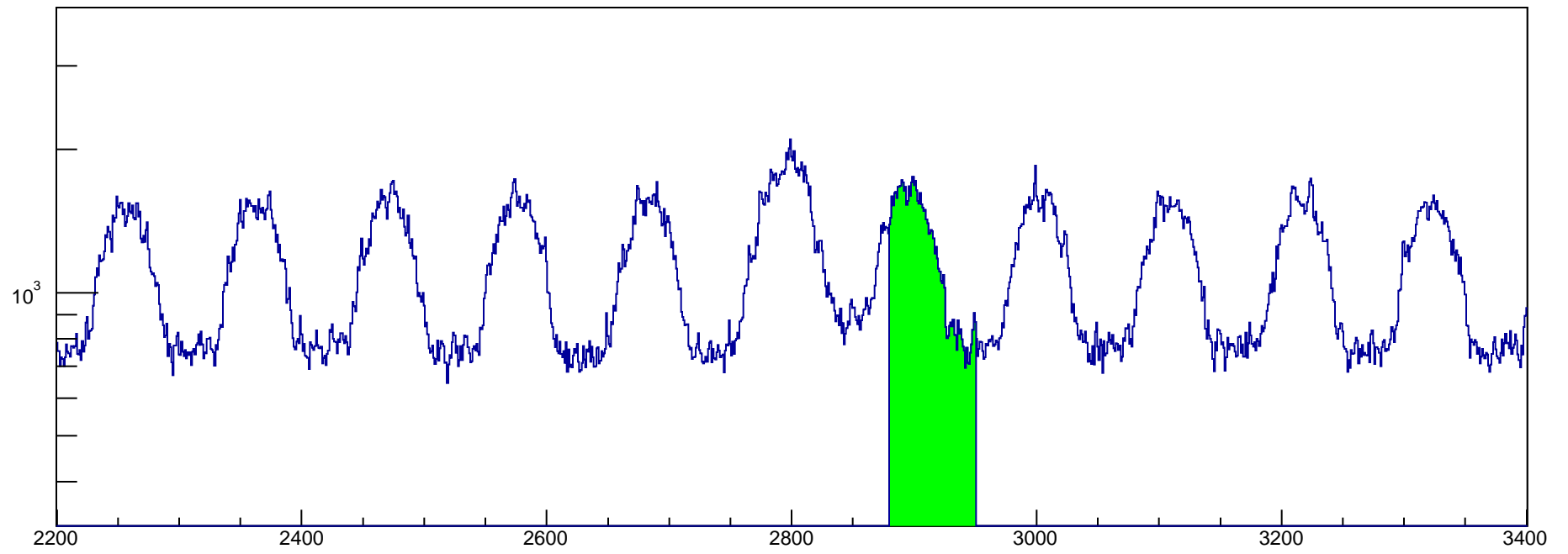
htrgdtme_mtd1
