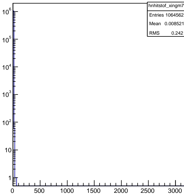
hnhitstof_xingm7
