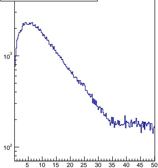
t-t_{\text{ear}}, n\text{Hits}/\text{tray}/\text{ev}>25
